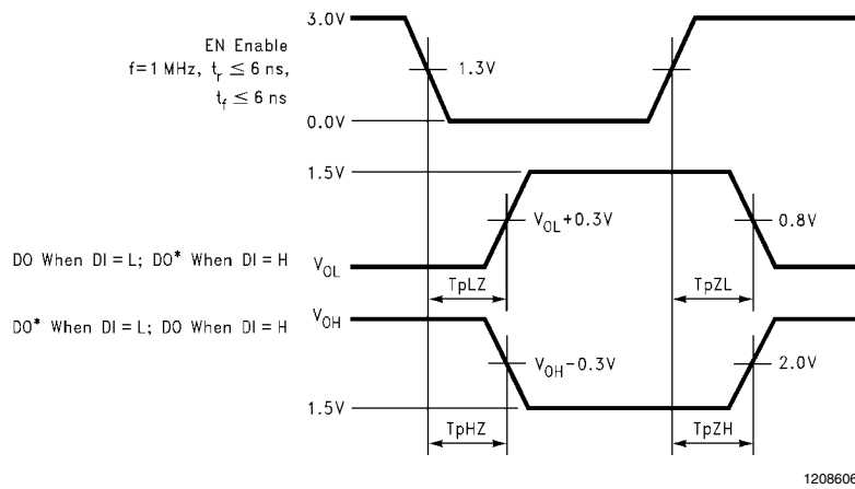
FIGURE 3. Enable and Disable Times
