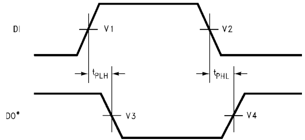
FIGURE 7. Propagation Delay Waveforms for Circuit 1 and Circuit 2 (See Figure 6)
