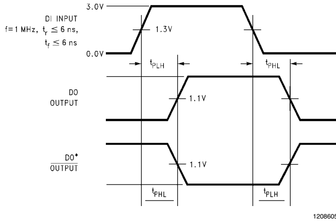
FIGURE 2. Propagation Delays
