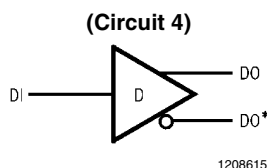
FIGURE 10. Circuit for Measuring Complementary Skew (See Figure 11)
