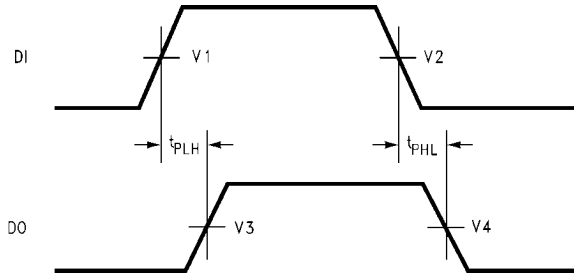
FIGURE 7. Propagation Delay Waveforms for Circuit 1 and Circuit 2 (See Figure 6)
